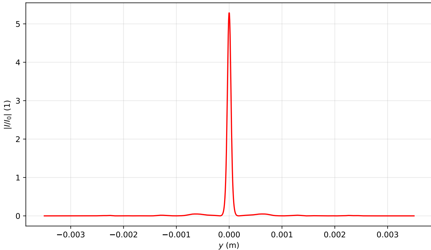
Intensity profile I(x=0, y, z=1.911)/I_0 , P_{in}=18.0\text{Pcr} , artificial time
