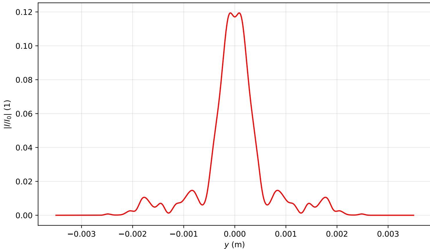
Intensity profile I(x=0, y, z=2.627)/I_0 , P_{in}=18.0P_{cr} , artificial time
