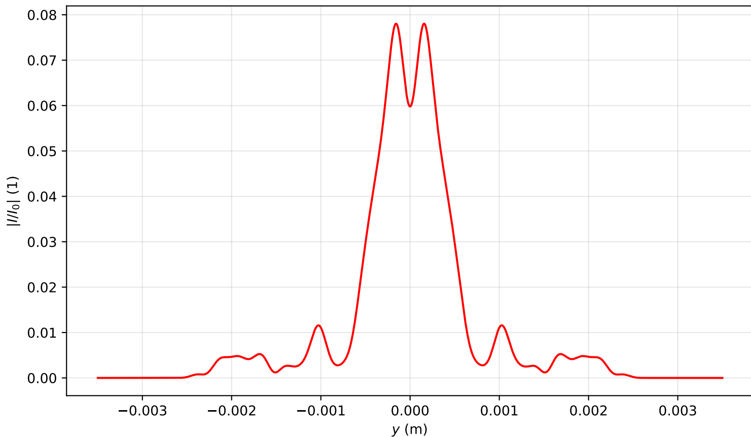
Intensity profile I(x=0, y, z=2.866)/I_0 , P_{in}=18.0P_{cr} , artificial time
