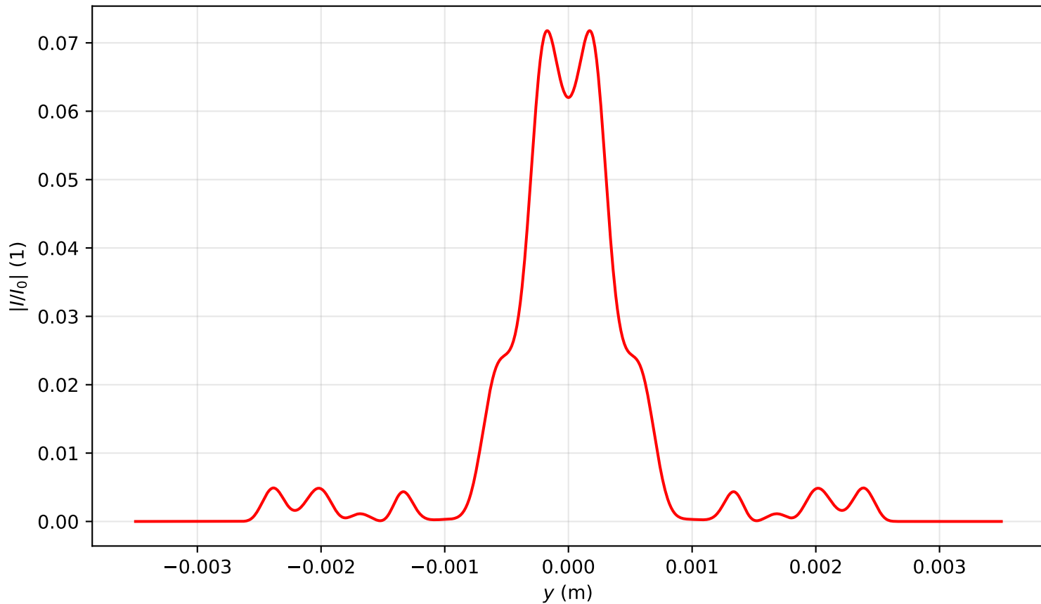
Intensity profile I(x=0, y, z=3.344)/I_0 , P_{in}=18.0\text{Pcr} , artificial time
