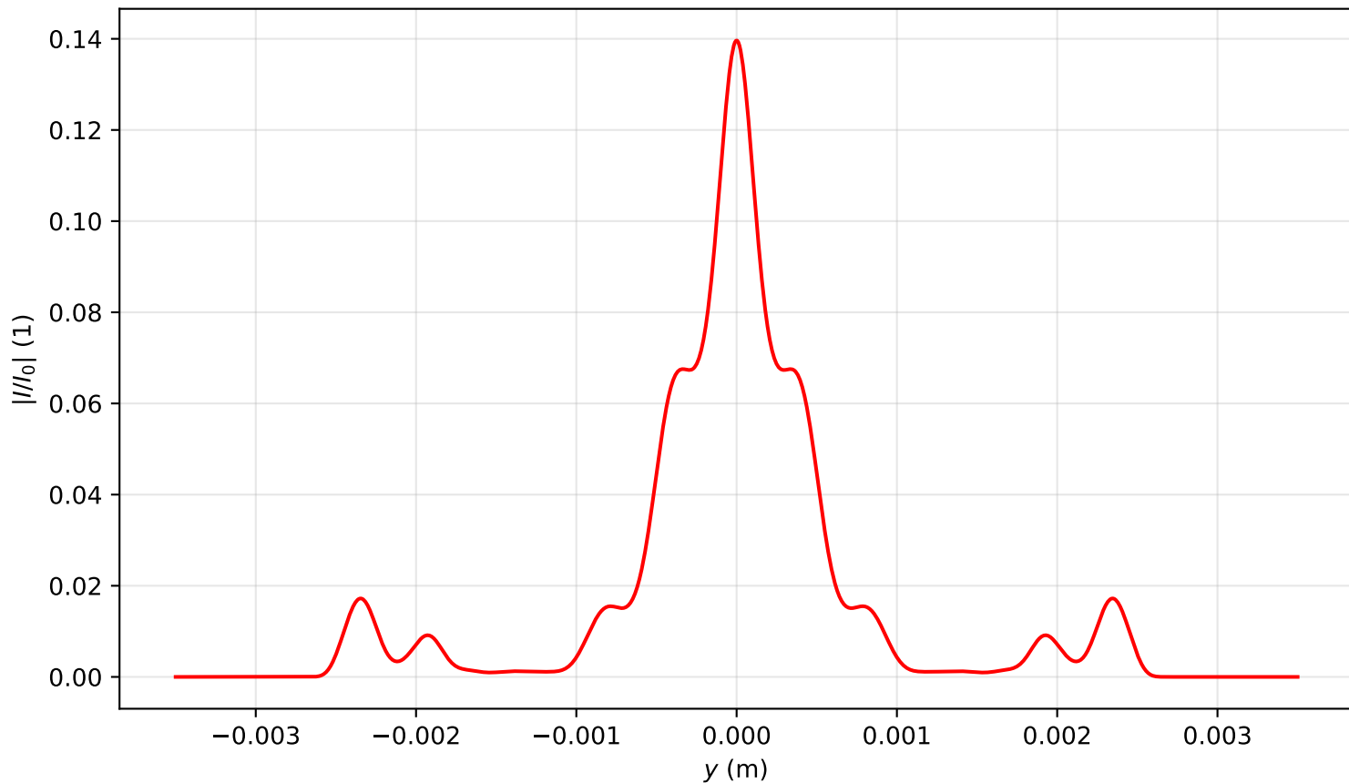
Intensity profile I(x=0, y, z=3.582)/I_0 , P_{in}=18.0P_{cr} , artificial time
