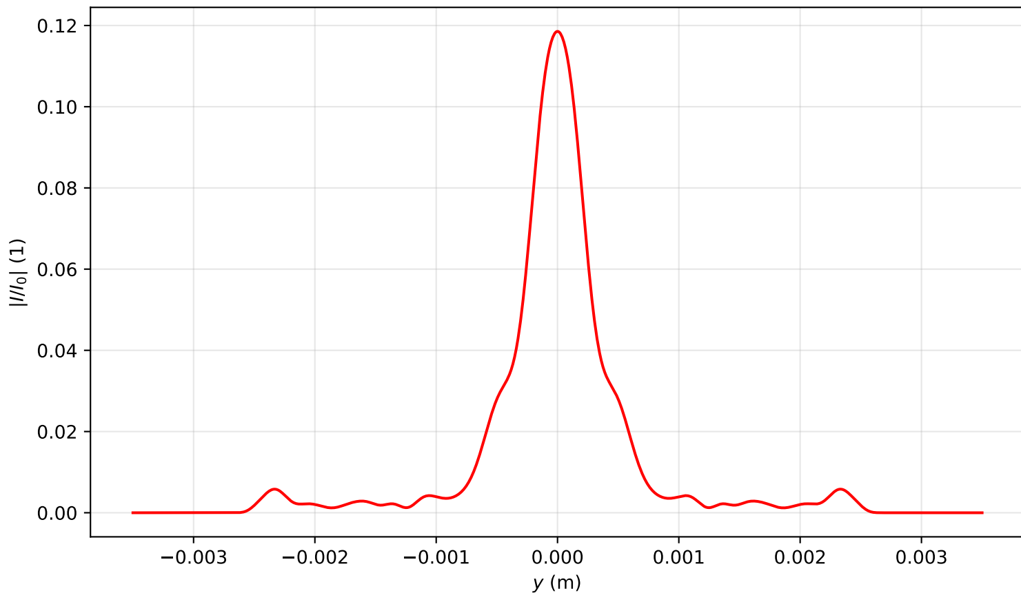
Intensity profile I(x=0, y, z=3.821)/I_0 , P_{in}=18.0\text{Pcr} , artificial time
