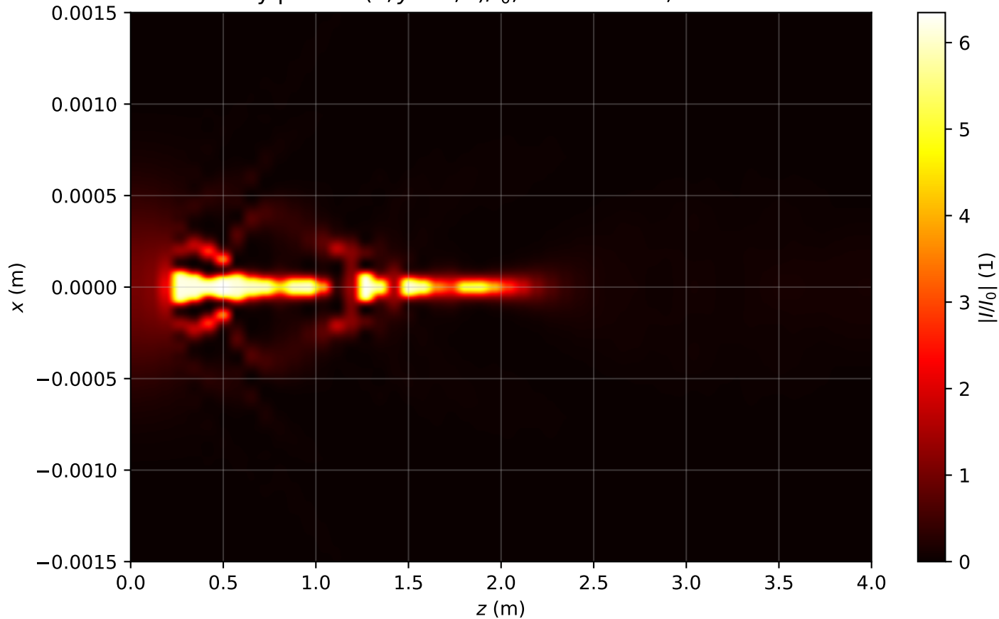
Intensity profile I(x, y = 0, z)/I_0 , P_{in}=18.0\text{Pcr} , artificial time
