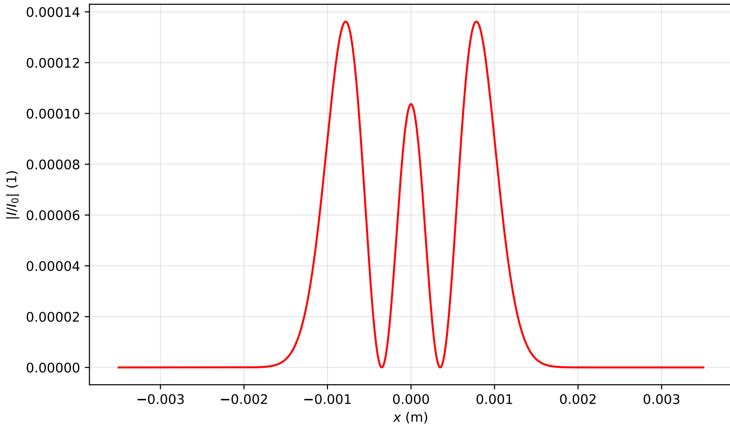
Intensity profile I(x, y = 0, z = 0.000)/I_0 , P_{in}=11.0P_{cr} , artificial time
