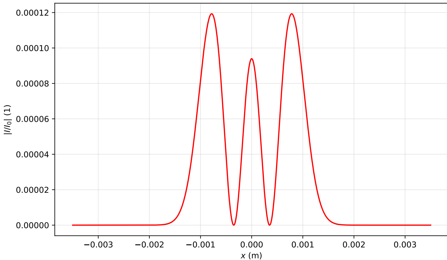
Intensity profile I(x, y = 0, z = 0.080)/I_0 , P_{in}=11.0P_{cr} , artificial time
