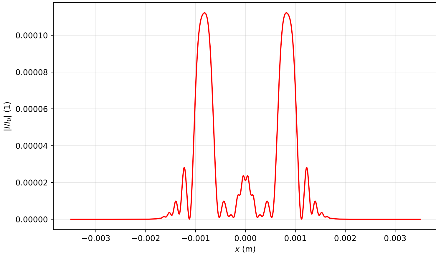
Intensity profile I(x, y = 0, z = 0.478)/I_0 , P_{in}=11.0P_{cr} , artificial time
