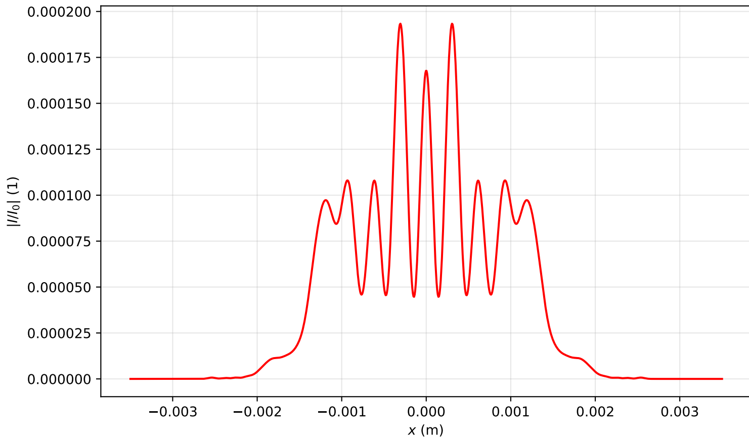
Intensity profile I(x, y = 0, z = 1.115)/I_0 , P_{in}=11.0P_{cr} , artificial time
