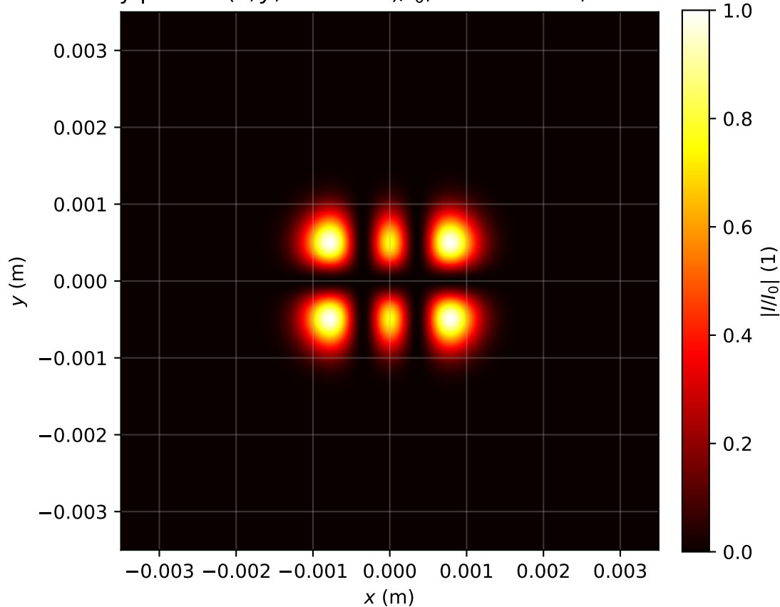
Intensity profile I(x, y, z = 0.000)/I_0 , P_{in}=11.0\text{Pcr} , artificial time
