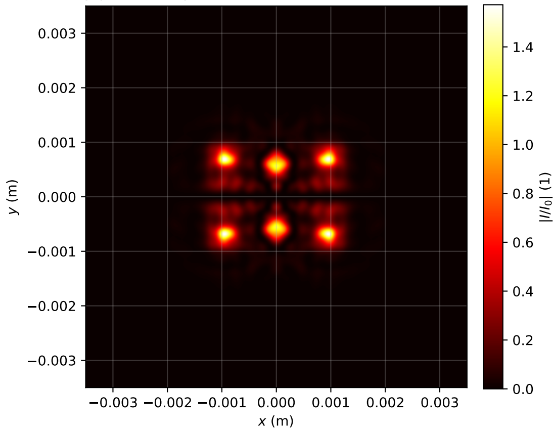
Intensity profile I(x, y, z = 1.035)/I_0 , P_{in}=11.0\text{Pcr} , artificial time
