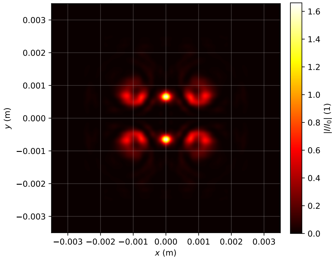
Intensity profile I(x, y, z = 1.831)/I_0 , P_{in}=11.0P_{cr} , artificial time
