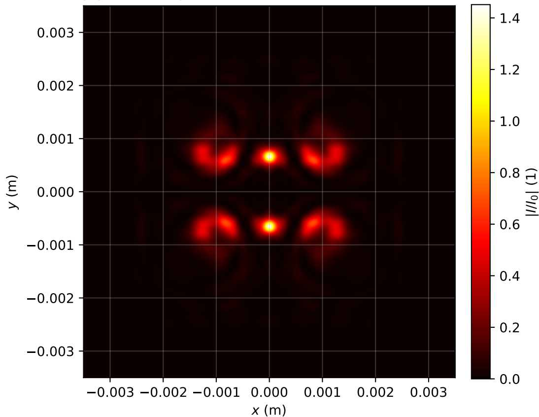
Intensity profile I(x, y, z = 1.911)/I_0 , P_{in}=11.0\text{Pcr} , artificial time
