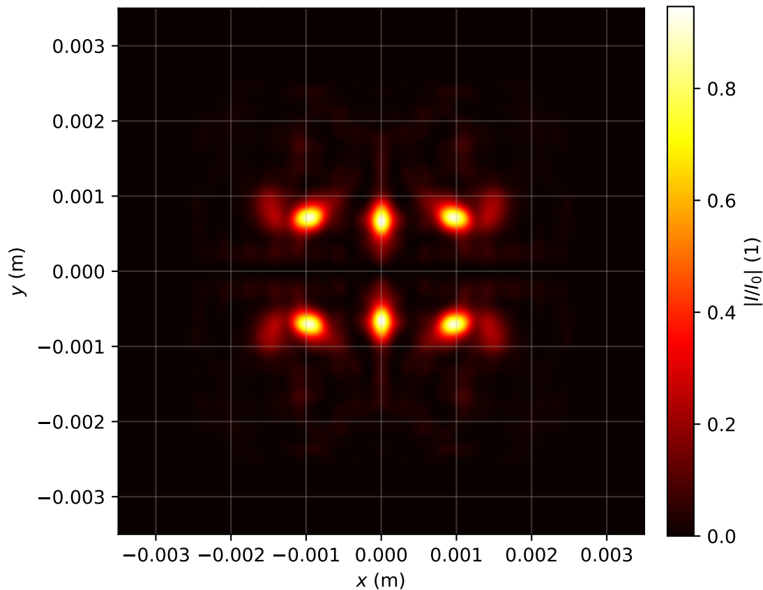
Intensity profile I(x, y, z = 2.229)/I_0 , P_{in}=11.0P_{cr} , artificial time
