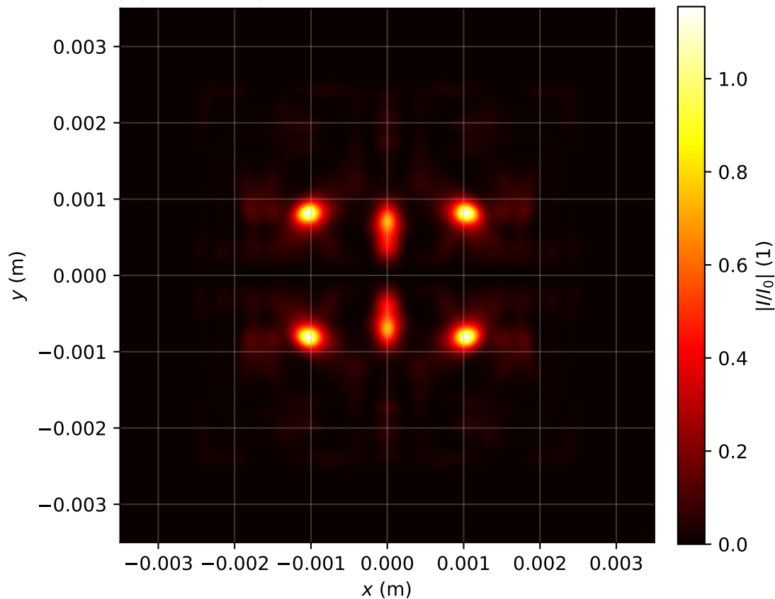
Intensity profile I(x, y, z = 2.468)/I_0 , P_{in}=11.0P_{cr} , artificial time
