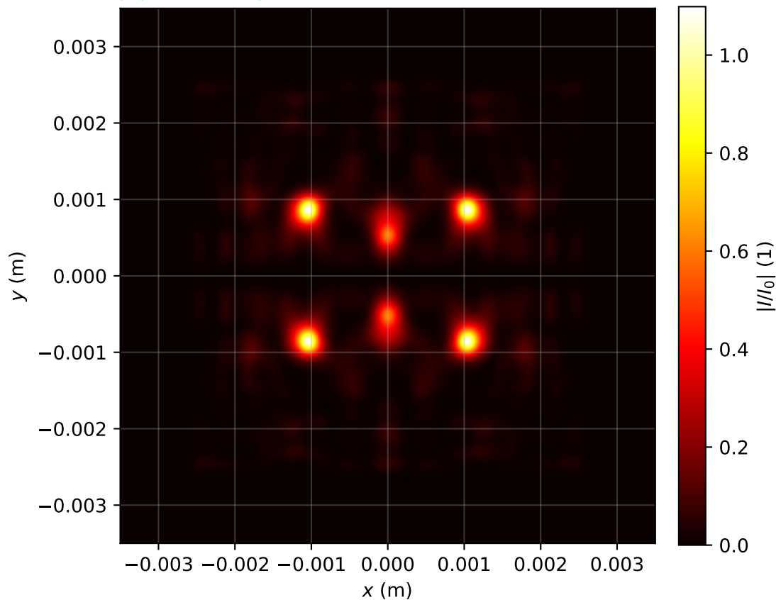
Intensity profile I(x, y, z = 2.627)/I_0 , P_{in}=11.0P_{cr} , artificial time
