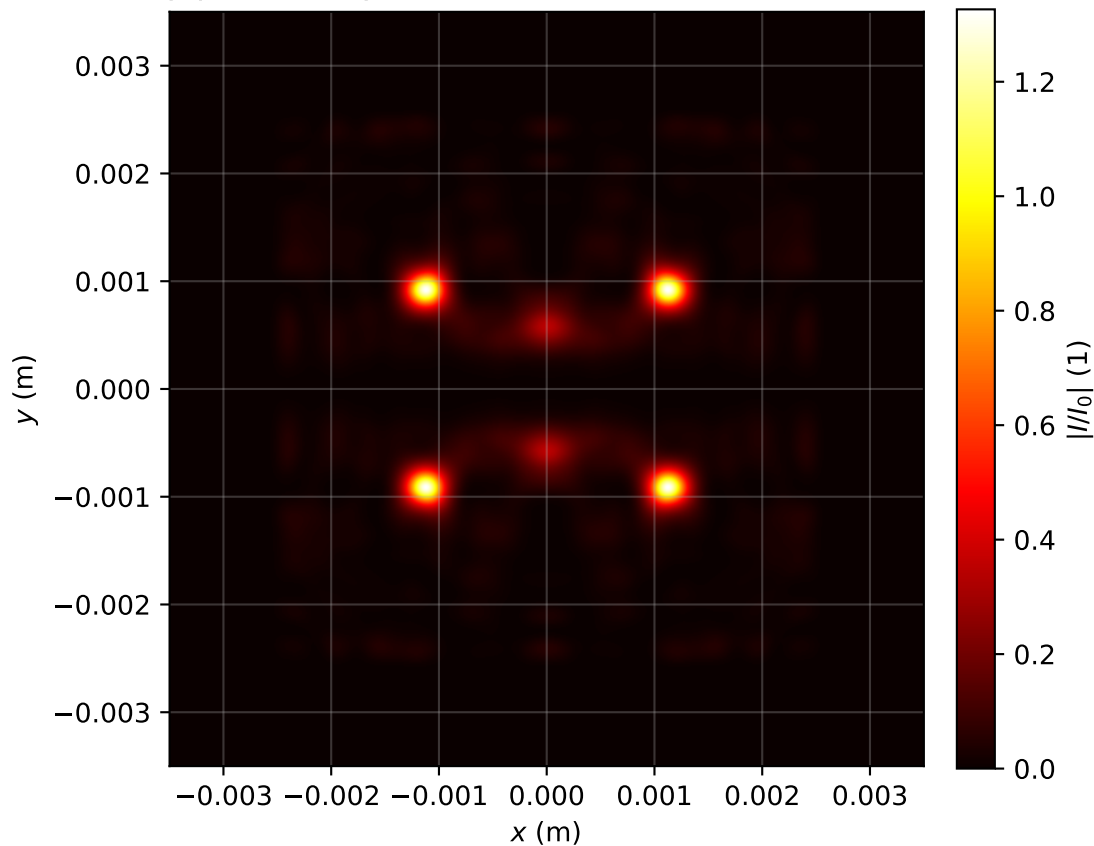
Intensity profile I(x, y, z = 3.105)/I_0 , P_{in}=11.0\text{Pcr} , artificial time
