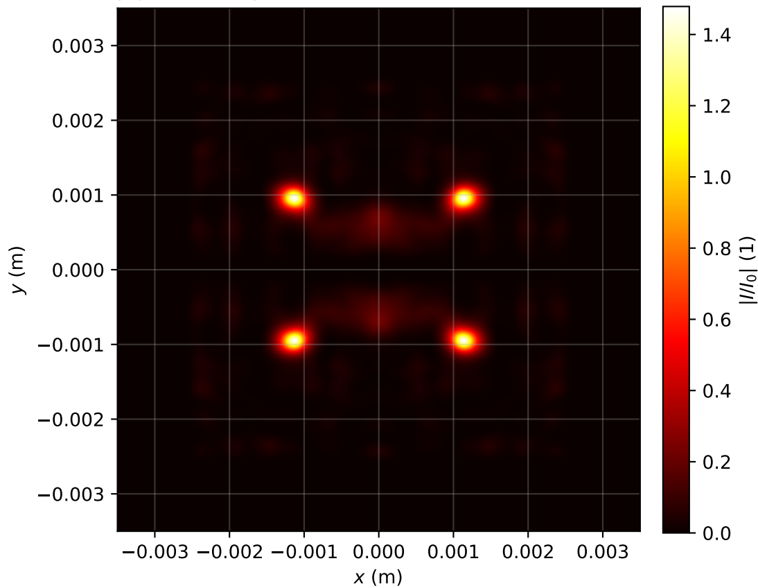
Intensity profile I(x, y, z = 3.264)/I_0 , P_{in}=11.0\text{Pcr} , artificial time
