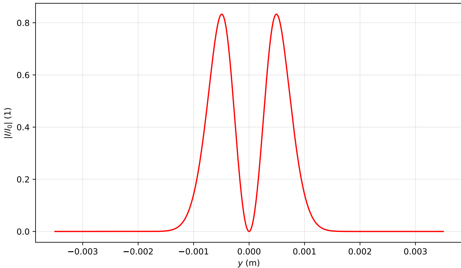
Intensity profile I(x=0, y, z=0.080)/I_0 , P_{in}=11.0P_{cr} , artificial time
