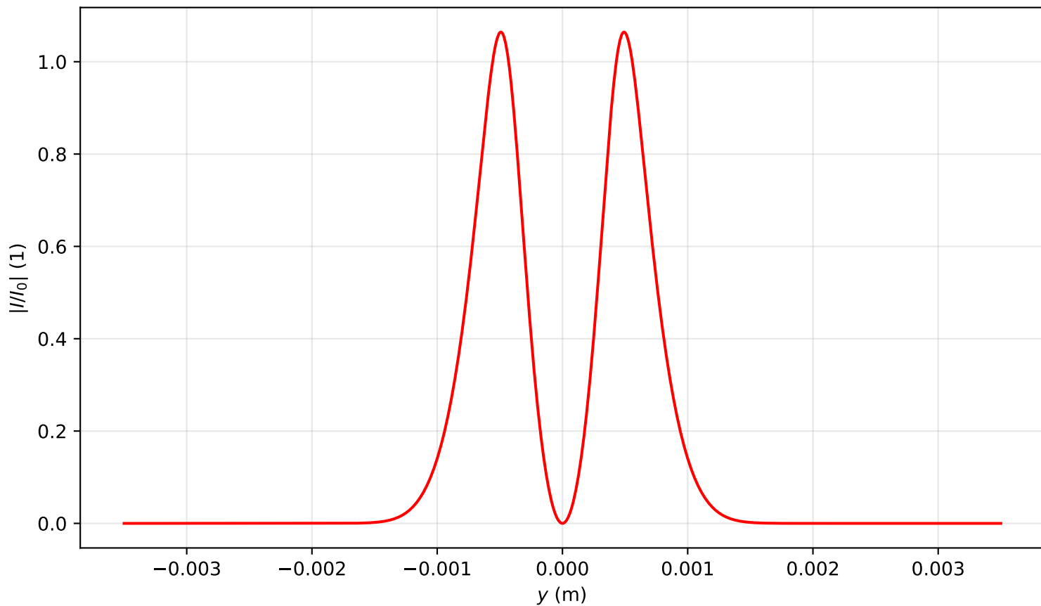
Intensity profile I(x=0, y, z=0.159)/I_0 , P_{in}=11.0P_{cr} , artificial time
