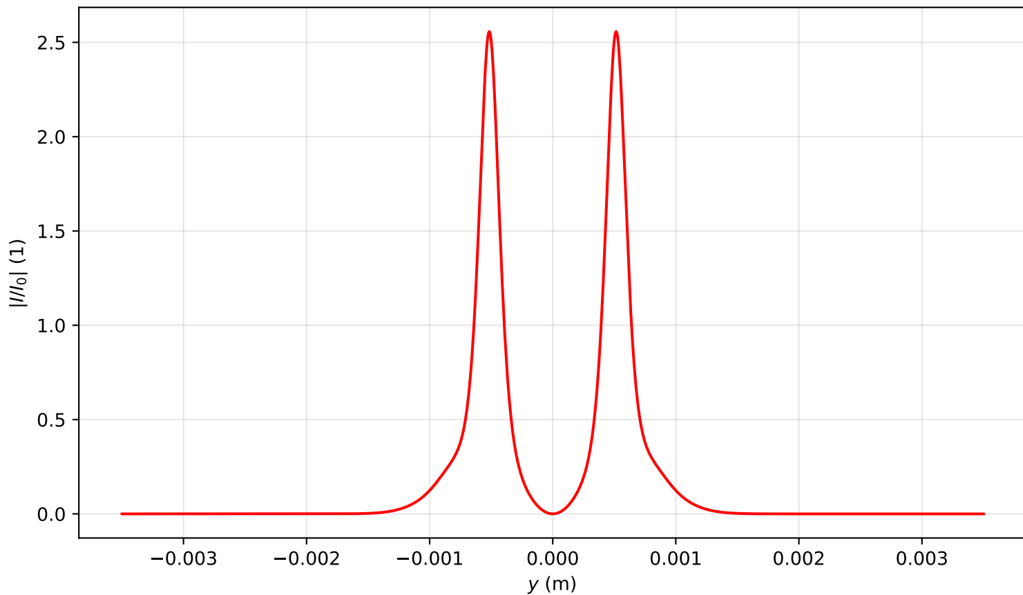
Intensity profile I(x=0, y, z=0.398)/I_0 , P_{in}=11.0P_{cr} , artificial time
