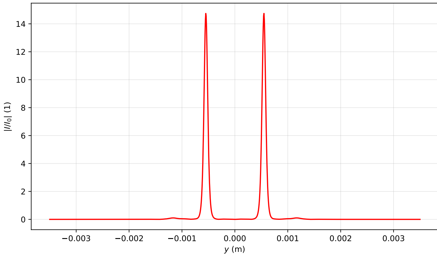
Intensity profile I(x=0, y, z=0.796)/I_0 , \text{Pin}=11.0\text{Pcr} , artificial time
