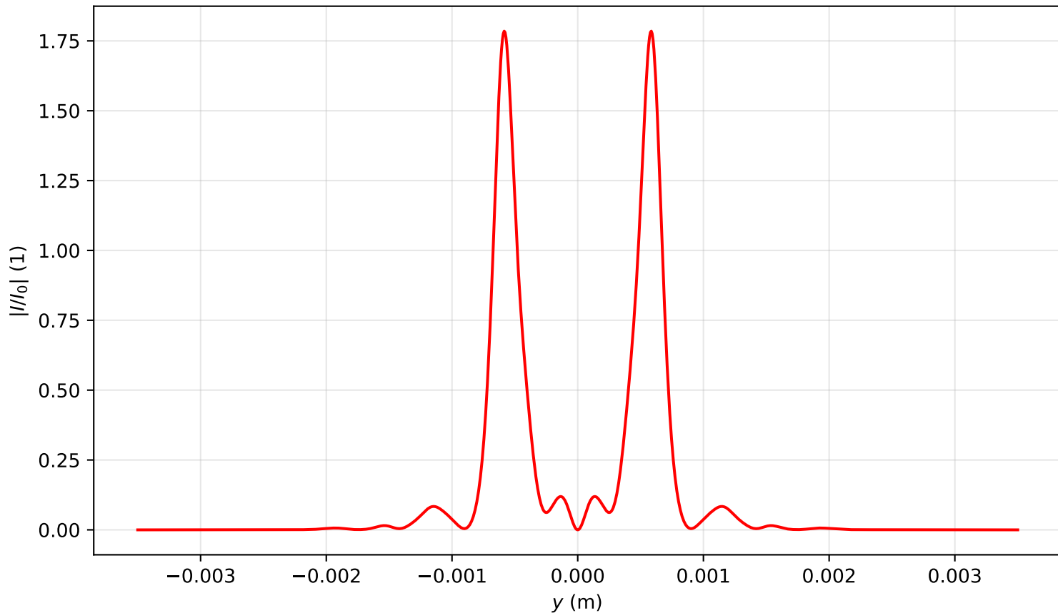
Intensity profile I(x=0, y, z=0.955)/I_0 , P_{in}=11.0\text{Pcr} , artificial time
