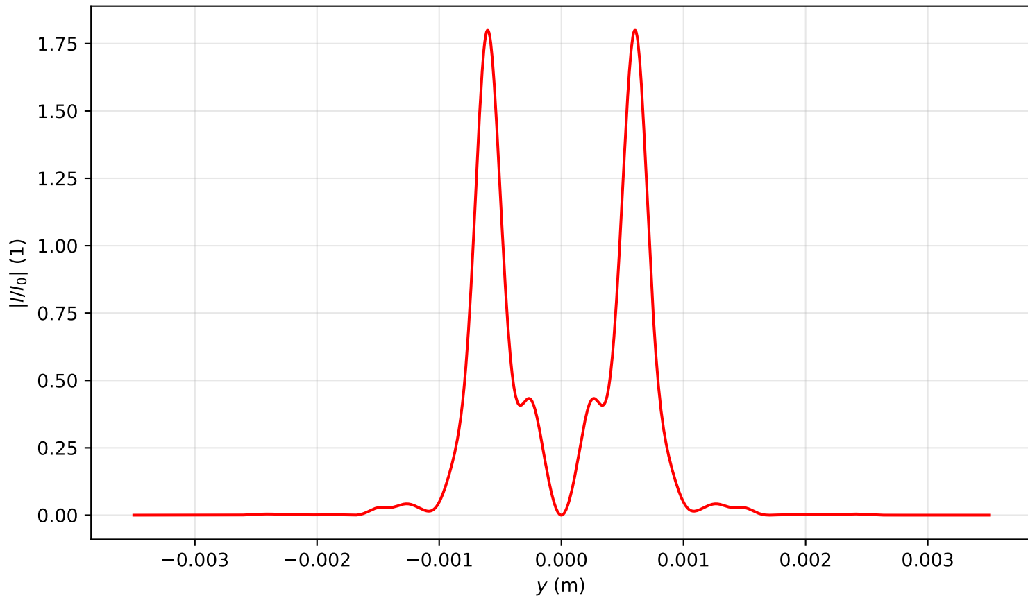
Intensity profile I(x=0, y, z=1.115)/I_0 , P_{in}=11.0P_{cr} , artificial time
