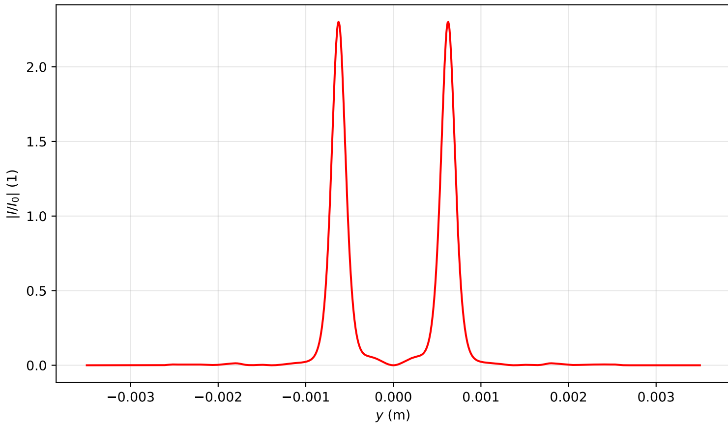
Intensity profile I(x=0, y, z=1.513)/I_0 , P_{in}=11.0P_{cr} , artificial time
