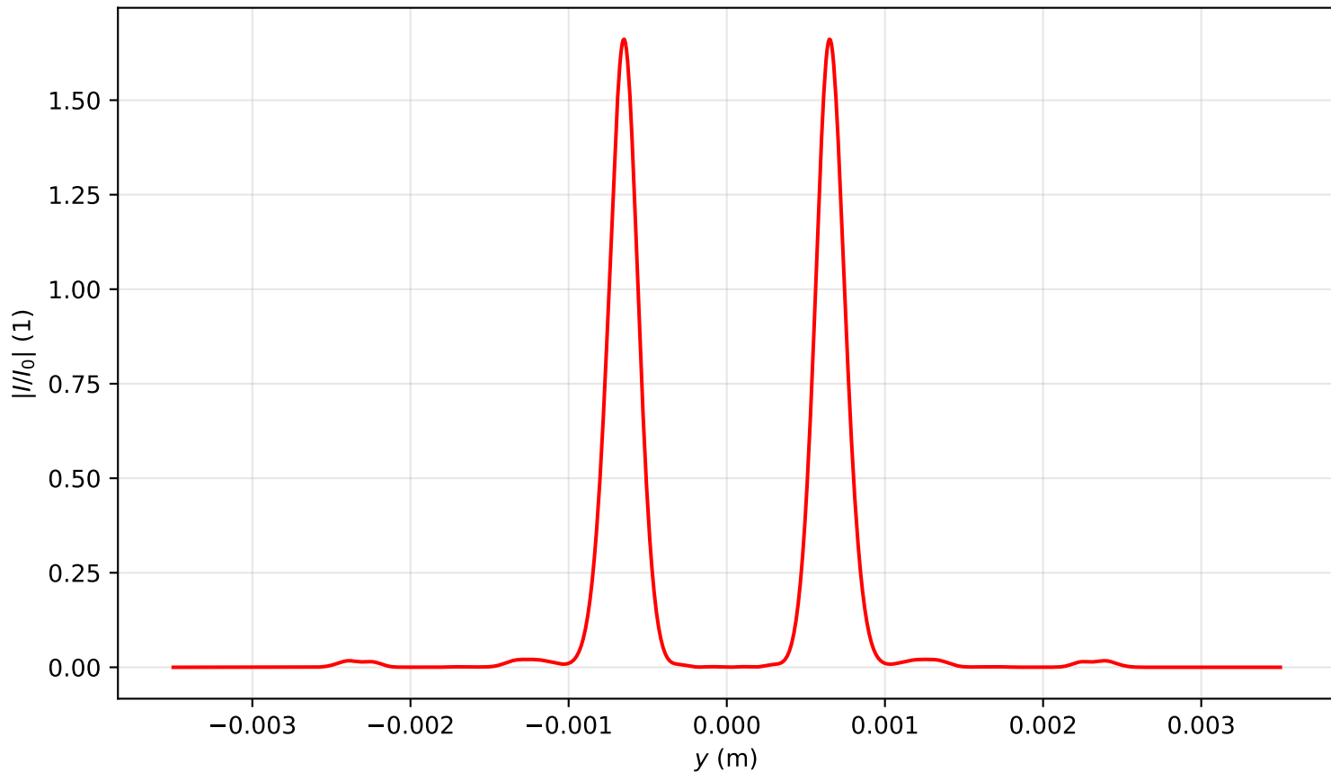
Intensity profile I(x=0, y, z=1.831)/I_0 , P_{in}=11.0P_{cr} , artificial time
