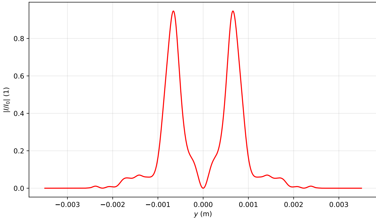
Intensity profile I(x=0, y, z=2.229)/I_0 , P_{in}=11.0P_{cr} , artificial time
