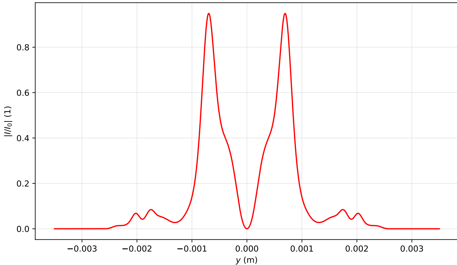
Intensity profile I(x=0, y, z=2.388)/I_0 , P_{in}=11.0P_{cr} , artificial time
