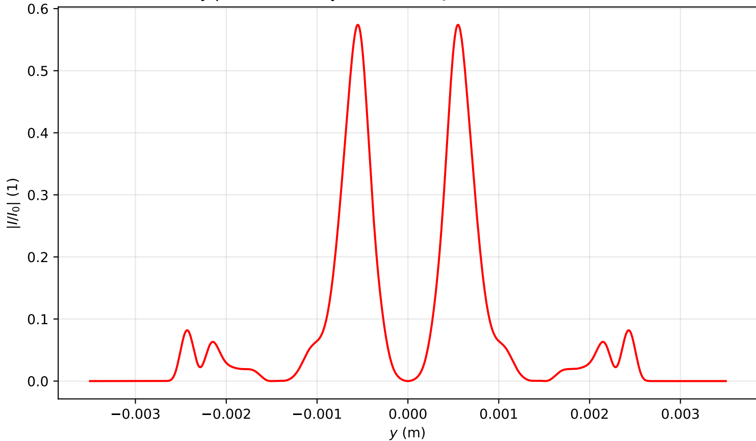
Intensity profile I(x=0, y, z=2.786)/I_0 , P_{in}=11.0P_{cr} , artificial time
