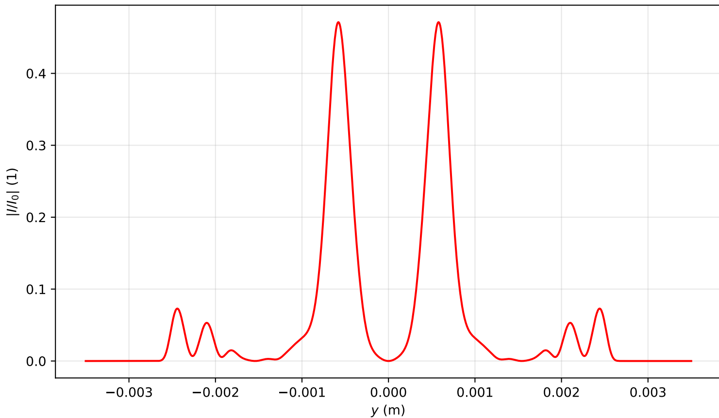
Intensity profile I(x=0, y, z=2.946)/I_0 , P_{in}=11.0P_{cr} , artificial time
