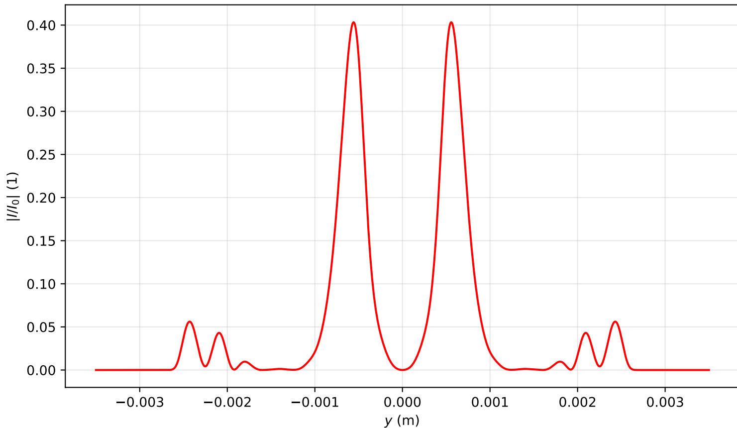
Intensity profile I(x=0, y, z=3.025)/I_0 , P_{in}=11.0P_{cr} , artificial time
