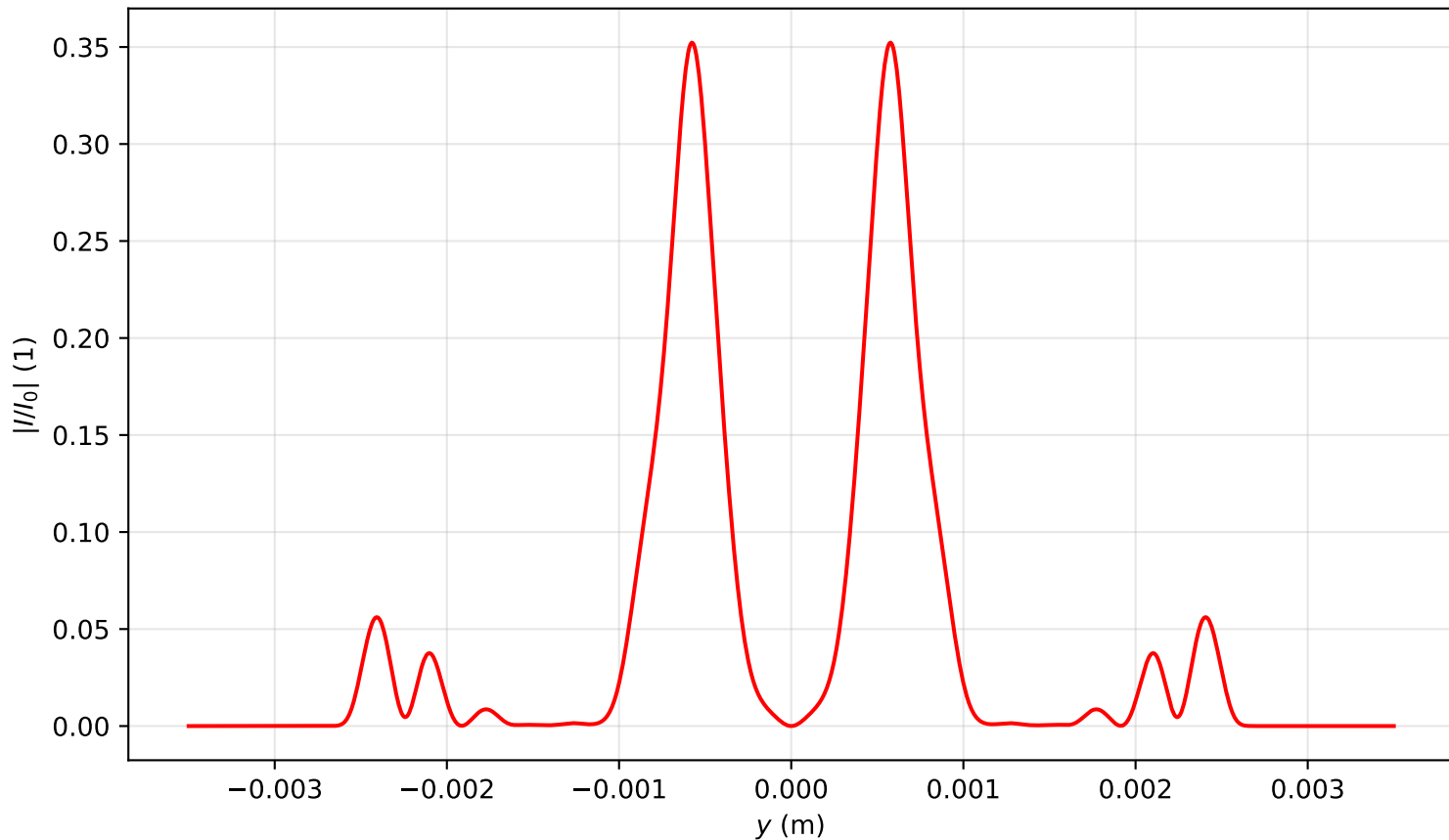
Intensity profile I(x=0, y, z=3.105)/I_0 , P_{in}=11.0P_{cr} , artificial time
