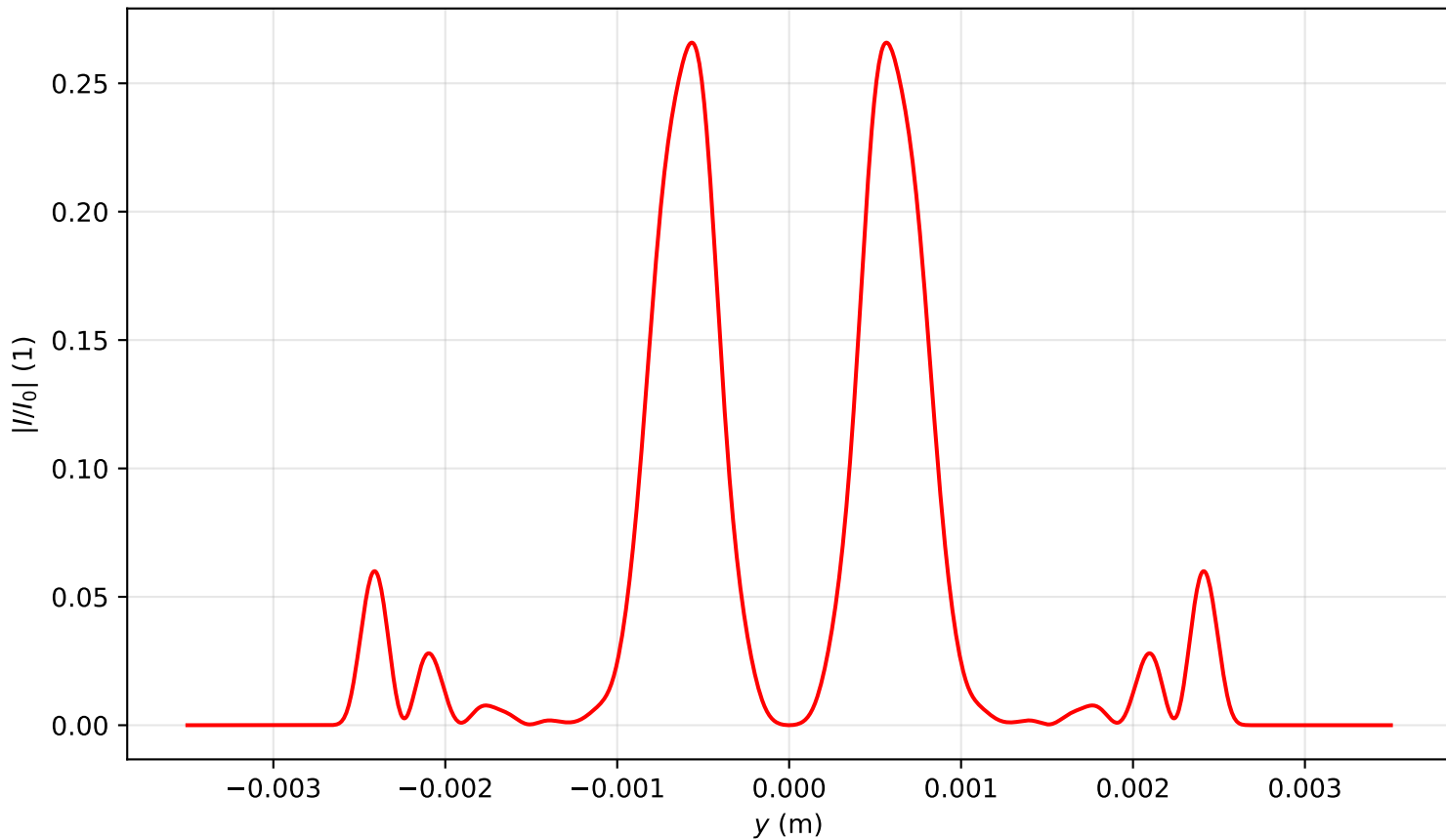
Intensity profile I(x=0, y, z=3.184)/I_0 , P_{in}=11.0P_{cr} , artificial time
