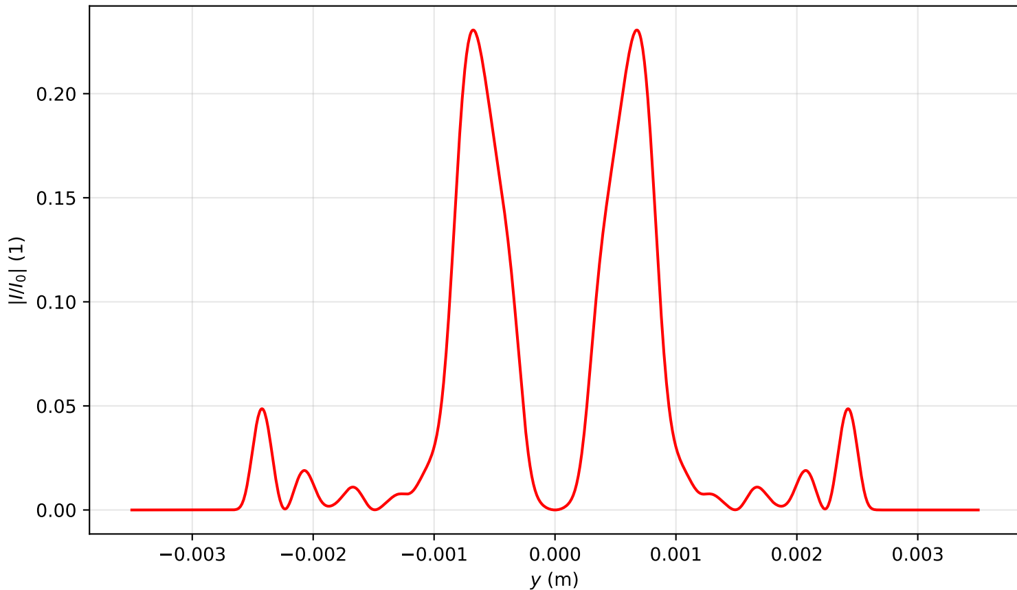
Intensity profile I(x=0, y, z=3.264)/I_0 , P_{in}=11.0P_{cr} , artificial time
