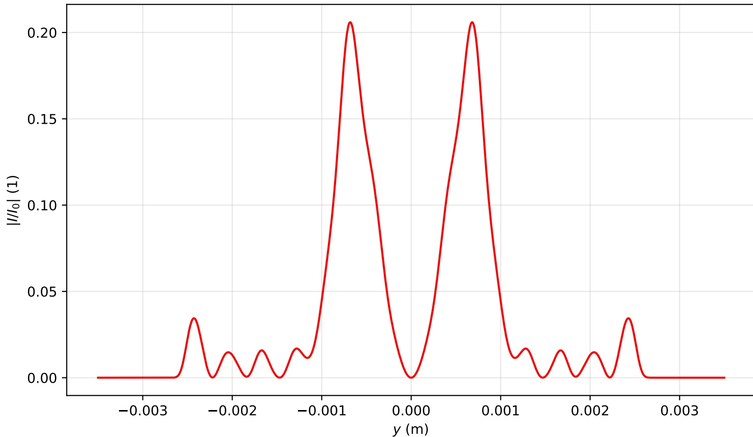
Intensity profile I(x=0, y, z=3.344)/I_0 , P_{in}=11.0P_{cr} , artificial time
