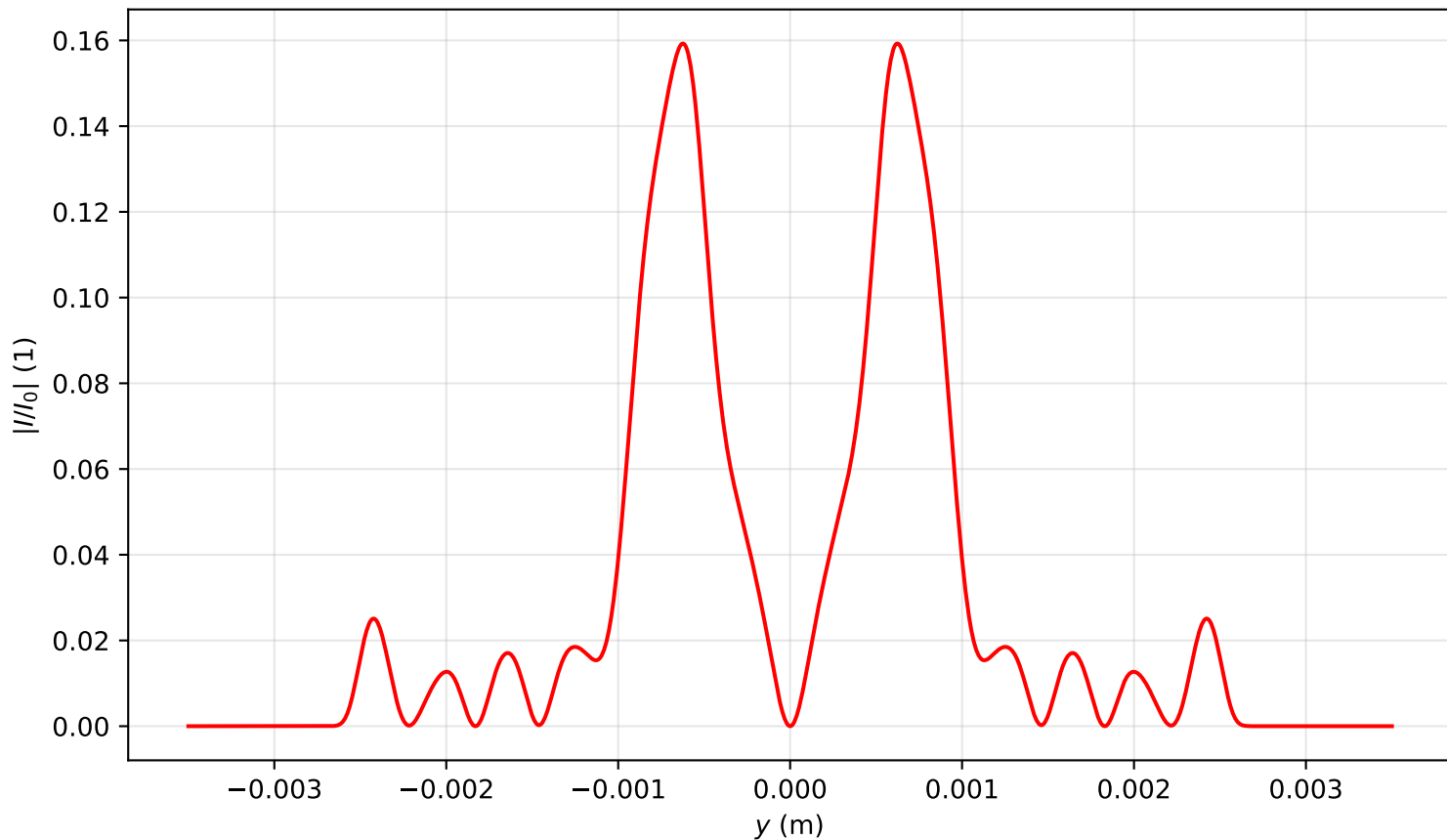
Intensity profile I(x=0, y, z=3.423)/I_0 , P_{in}=11.0P_{cr} , artificial time
