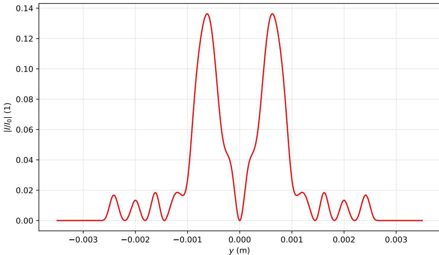
Intensity profile I(x=0, y, z=3.503)/I_0 , P_{in}=11.0P_{cr} , artificial time
