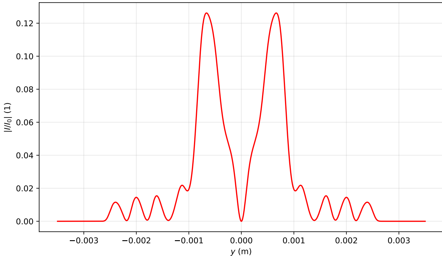
Intensity profile I(x=0, y, z=3.582)/I_0 , P_{in}=11.0P_{cr} , artificial time
