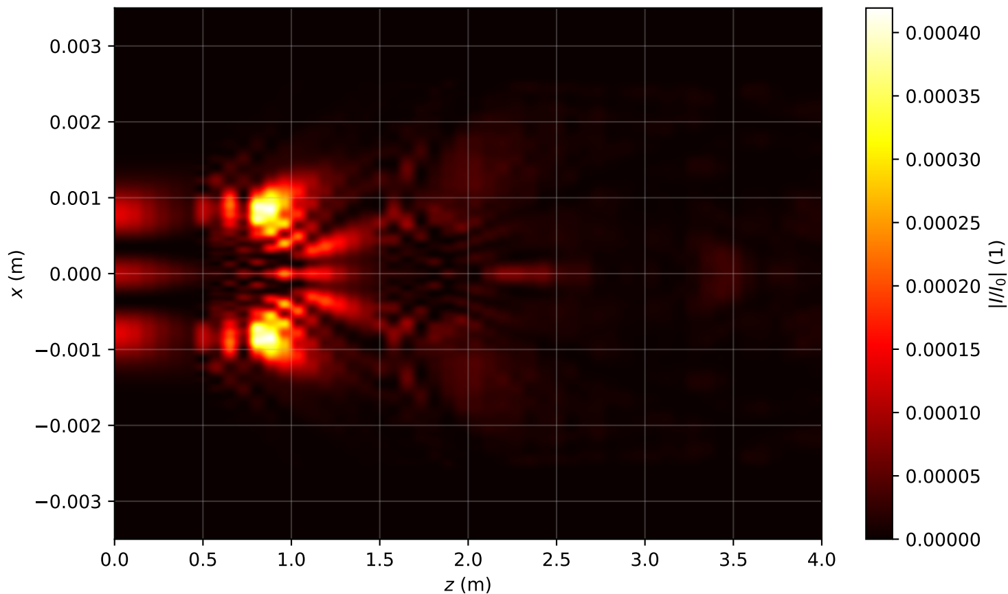
Intensity profile I(x, y = 0, z)/I_0 , P_{in}=11.0P_{cr} , artificial time
