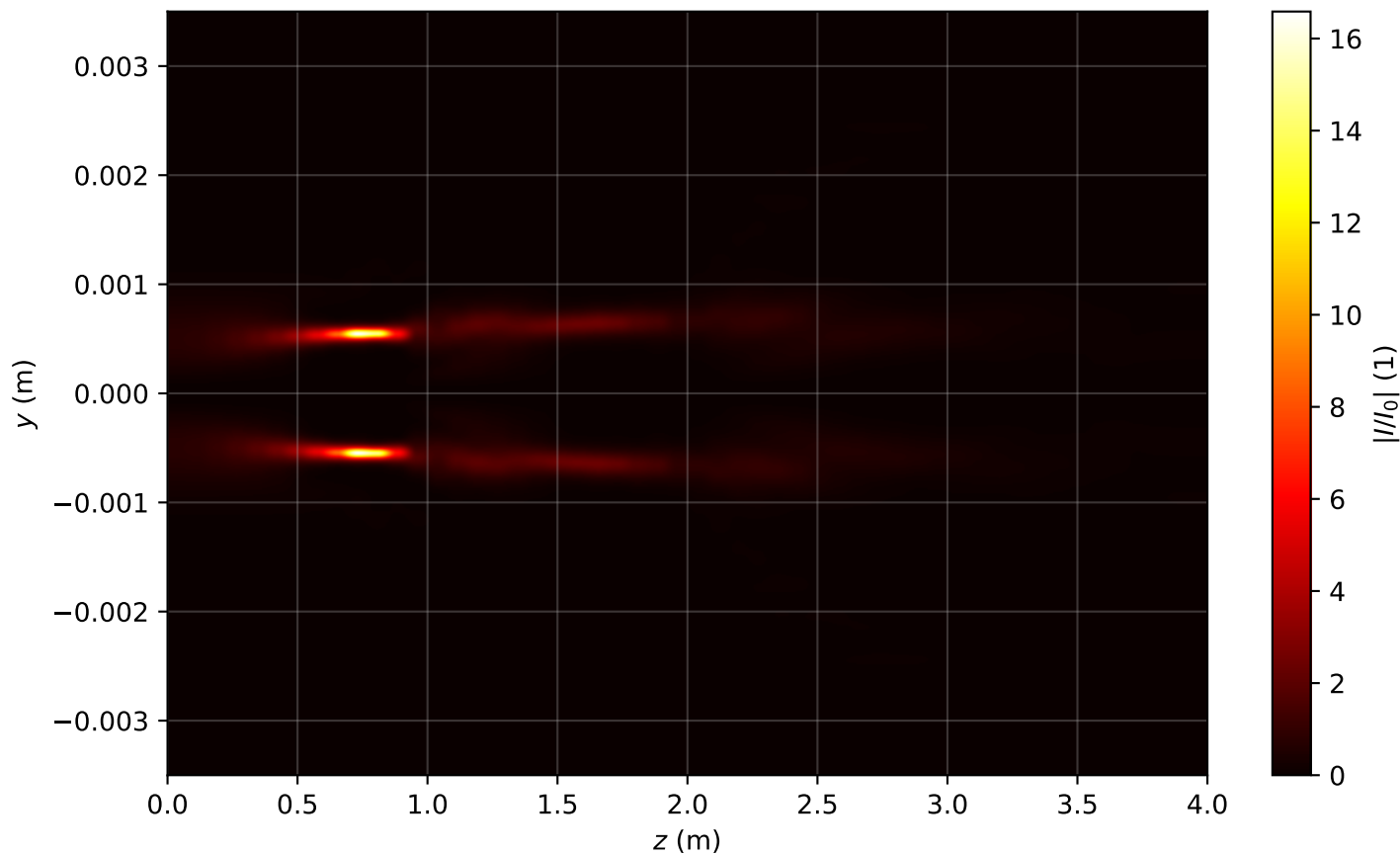
Intensity profile I(x = 0, y, z)/I_0 , P_{in}=11.0P_{cr} , artificial time
