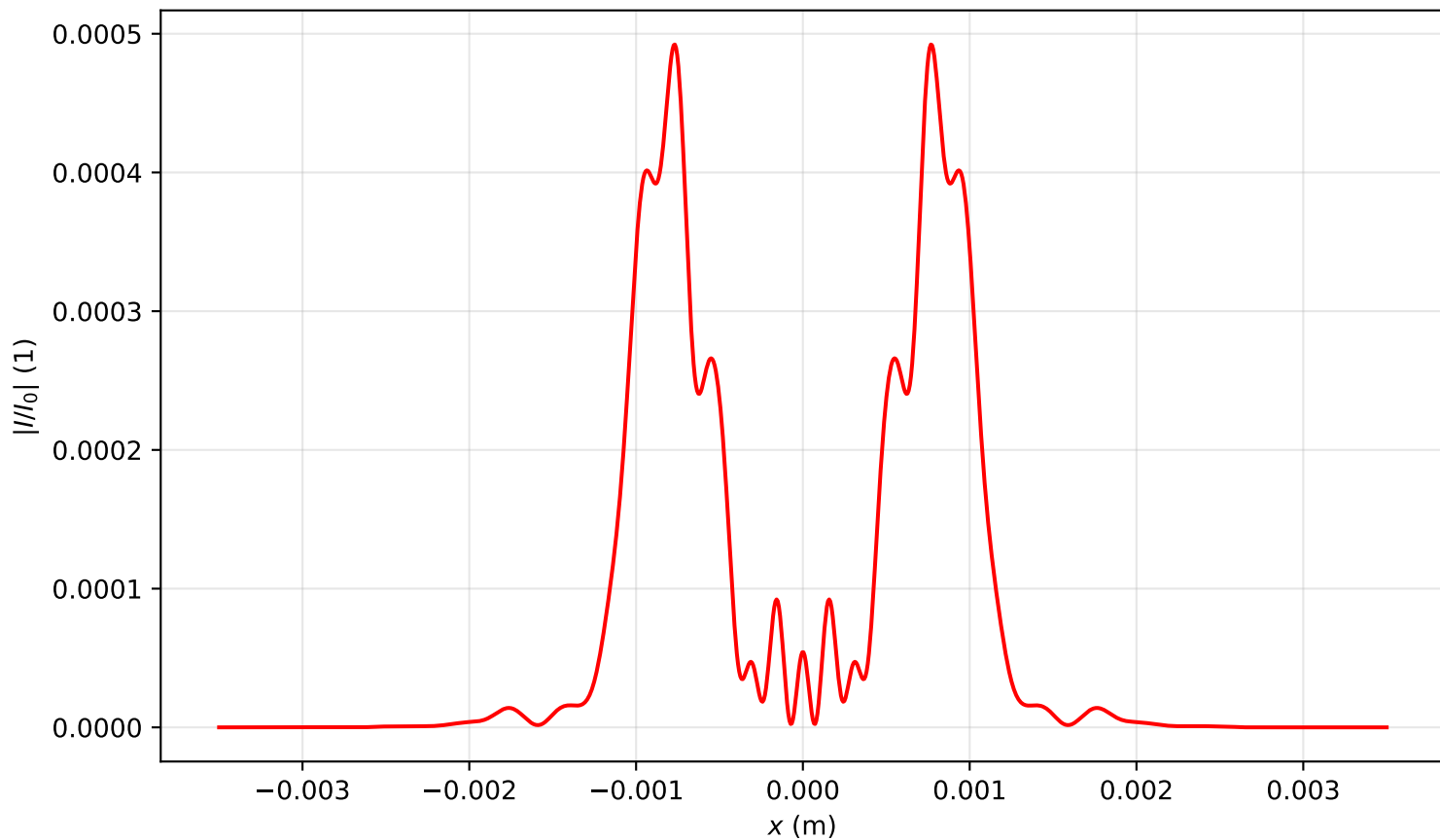
Intensity profile I(x, y = 0, z = 0.796)/I_0 , P_{in}=12.0P_{cr} , artificial time
