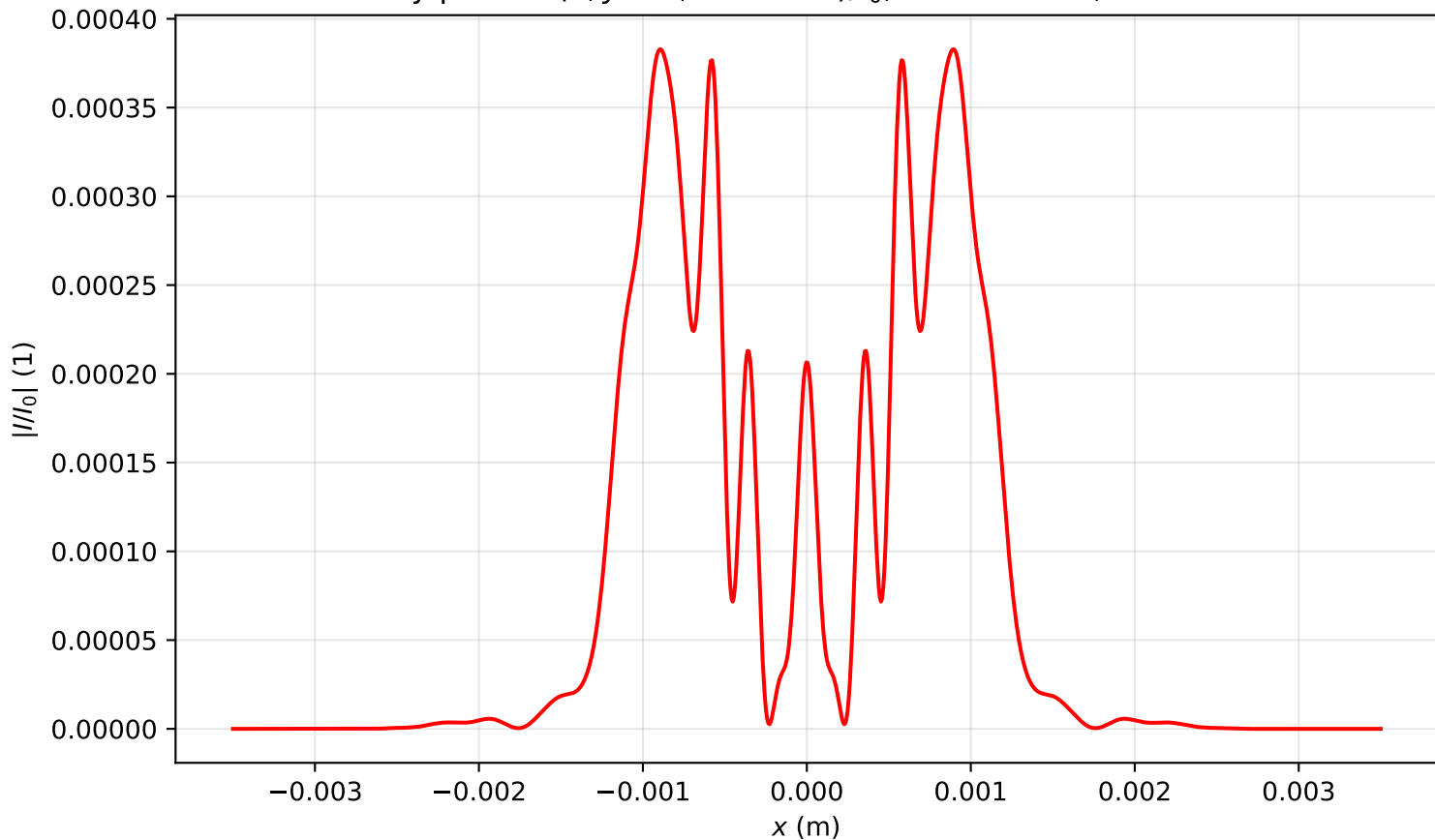
Intensity profile I(x, y = 0, z = 0.876)/I_0 , P_{in}=12.0P_{cr} , artificial time
