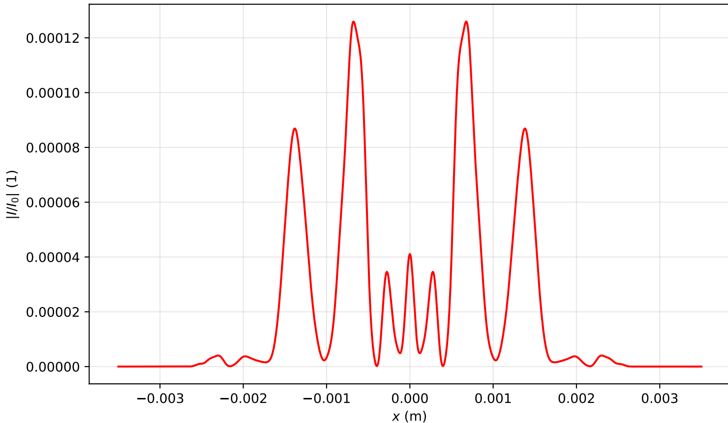
Intensity profile I(x, y = 0, z = 1.513)/I_0 , P_{in}=12.0P_{cr} , artificial time
