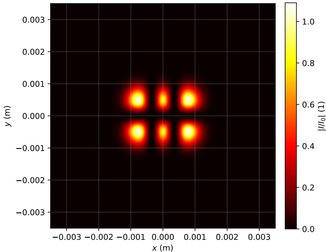
Intensity profile I(x, y, z = 0.080)/I_0 , P_{in}=12.0\text{Pcr} , artificial time
