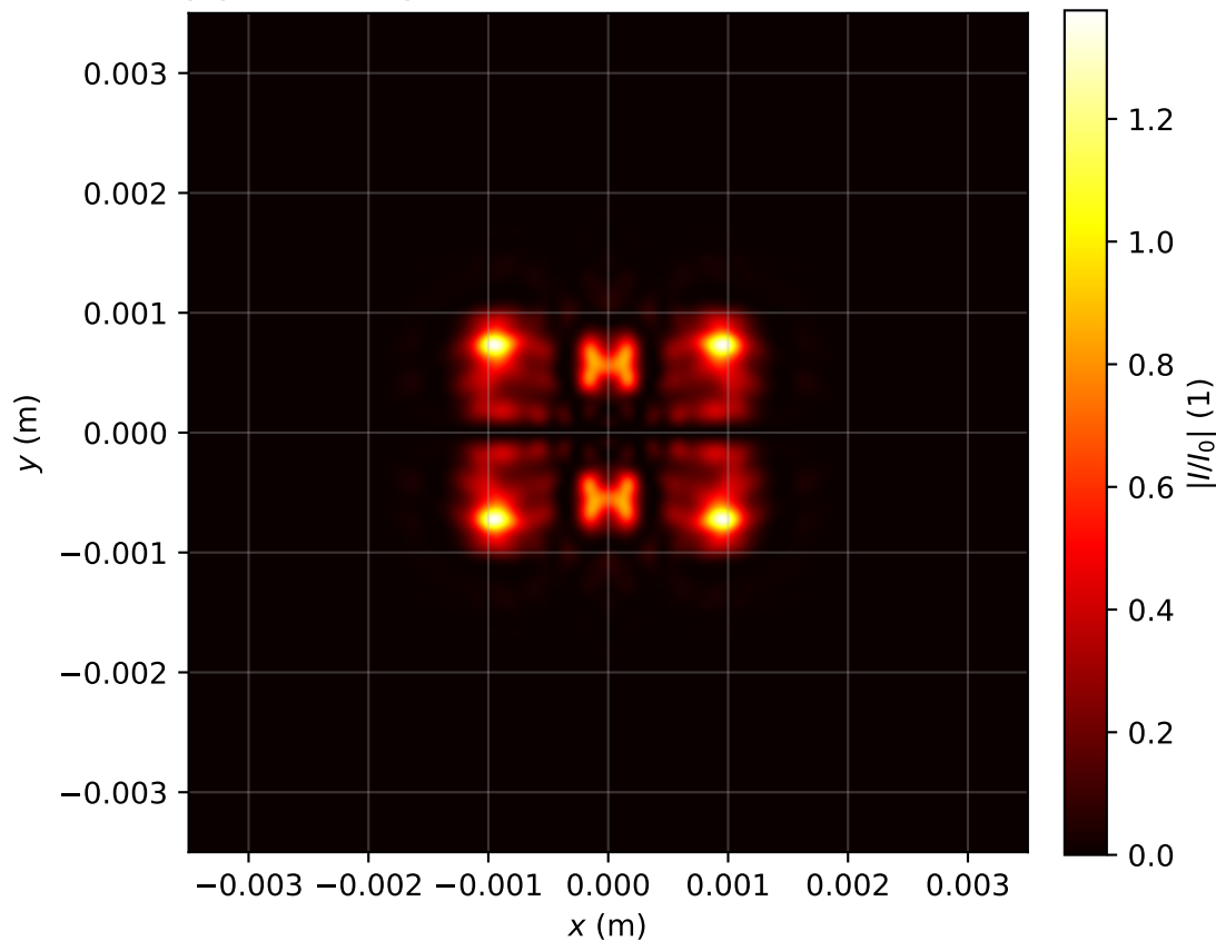
Intensity profile I(x, y, z = 0.876)/I_0 , P_{in}=12.0P_{cr} , artificial time
