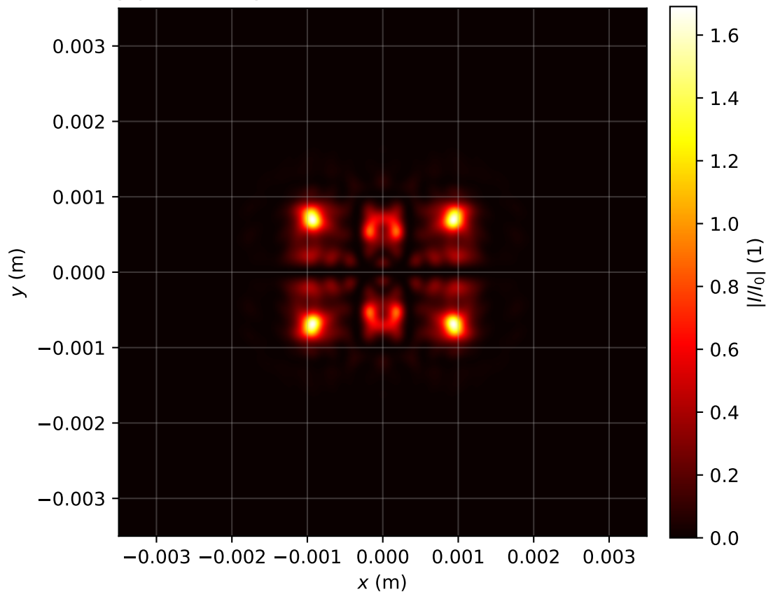
Intensity profile I(x, y, z = 0.955)/I_0 , P_{in}=12.0\text{Pcr} , artificial time
