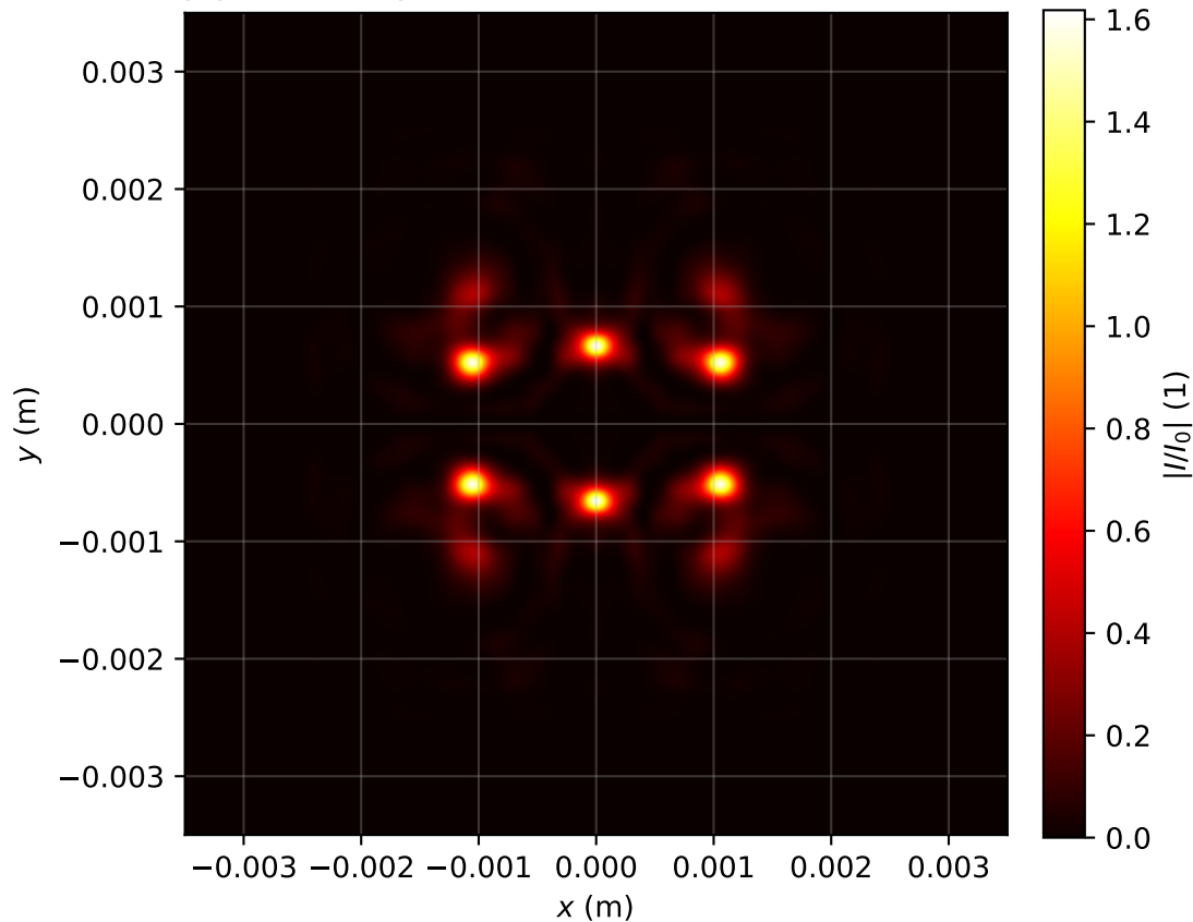
Intensity profile I(x, y, z = 1.751)/I_0 , P_{in}=12.0\text{Pcr} , artificial time
