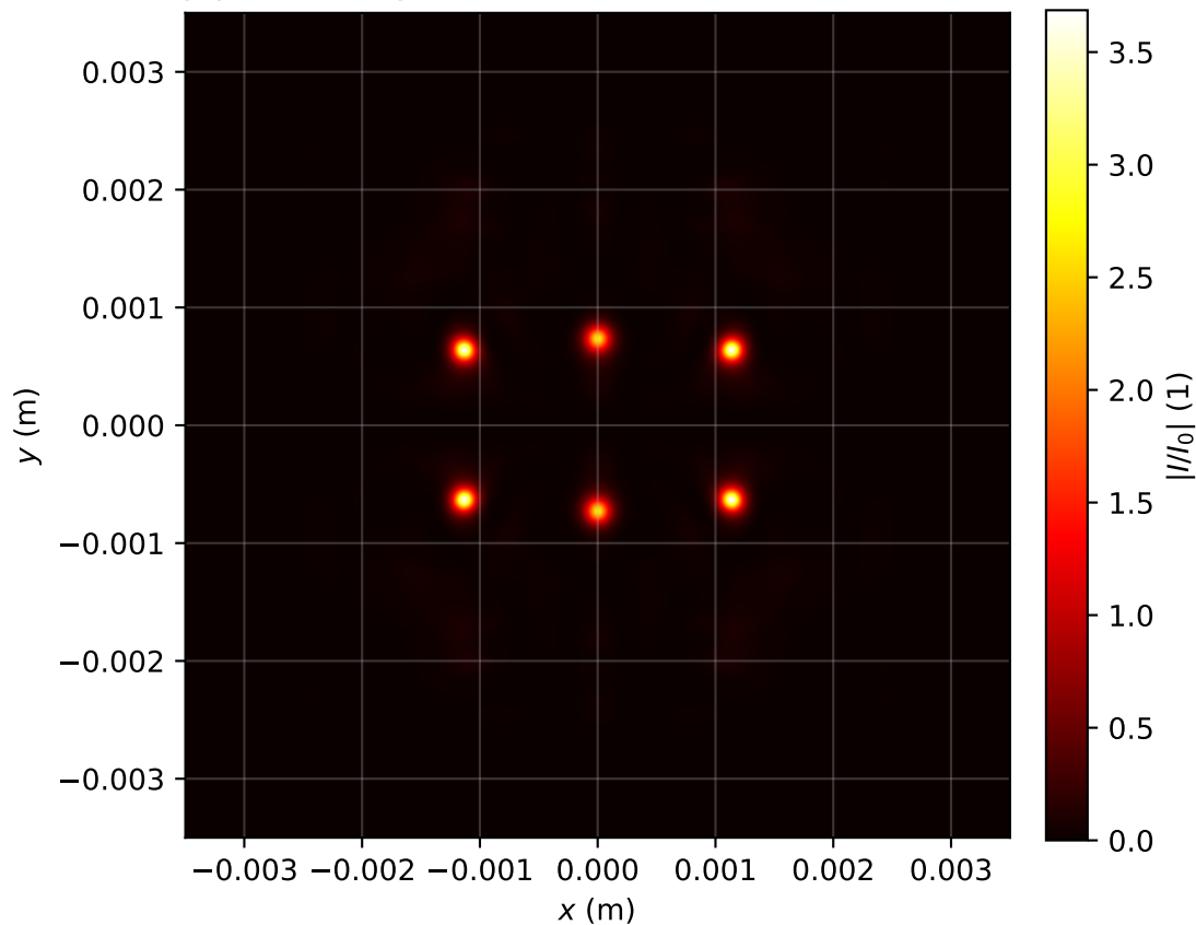
Intensity profile I(x, y, z = 2.309)/I_0 , P_{in}=12.0\text{Pcr} , artificial time
